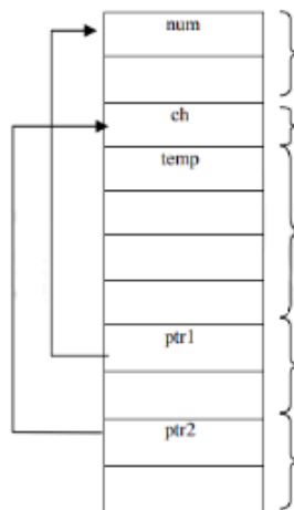
Concept of Pointer Variables
